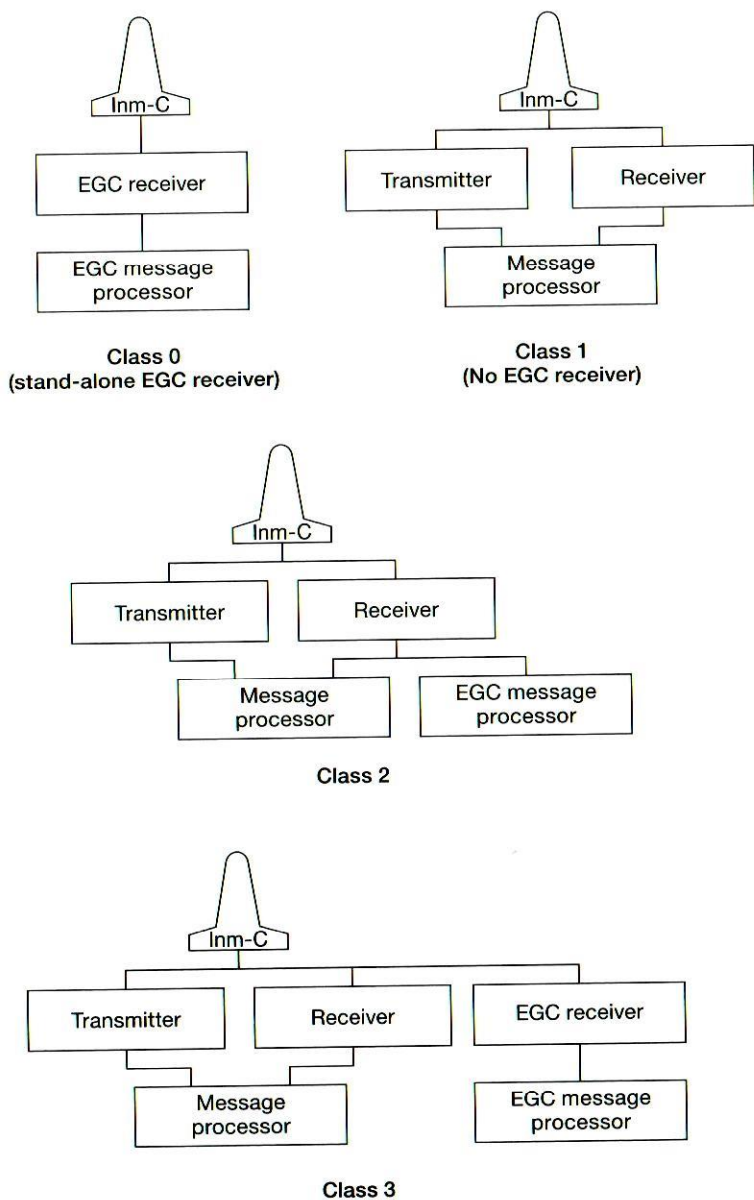
Figure 9 – Classes of Inmarsat-C Mobile Earth Stations
