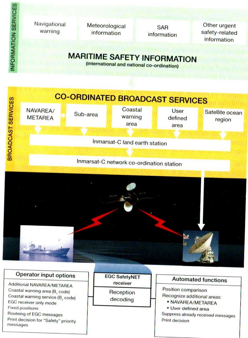
Figure 1 – The International SafetyNET Service system
