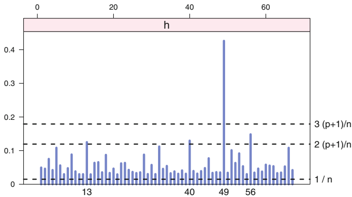
Fig. 11.12 Leverage for Model (11.1) for rent data.
