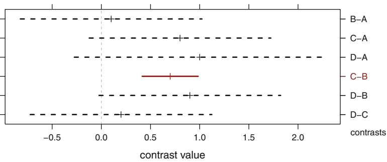
Fig. 7.10 Simultaneous confidence intervals on all pairs of mean differences. The means of samples B and C both lie between the means of samples A and D. Sample sizes were 100 from populations B and C and 5 from populations A and D. The Tukey procedure finds a significant difference between the means of populations B and C but no significant difference between the means of populations A and D. The short confidence interval for the C-A contrast reflects the higher precision of the contrasts based on the larger sample sizes.
