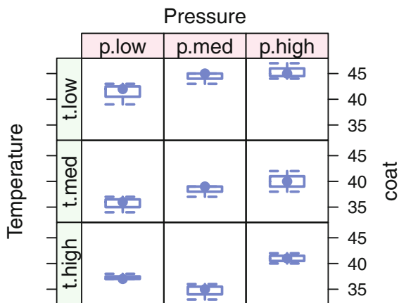
Fig. 13.8 a Filmcoat data. Each box is based on three data points. The interaction between temperature and pressure is very visible in the t.high \sim p.med panel. Along the top two rows of the plot, the boxes move up from left to right. In the bottom row, the second box is below the other two.
