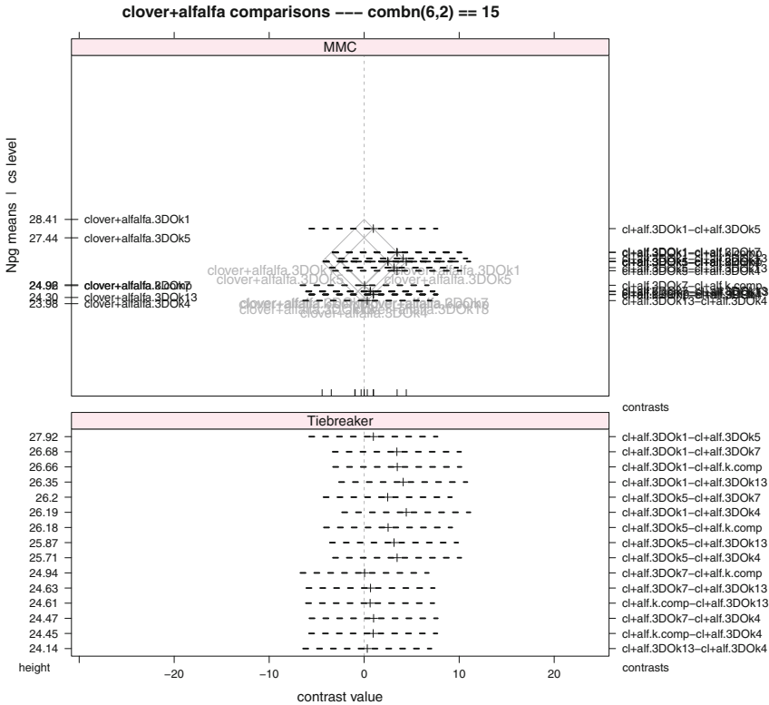
Fig. 12.16 MMC plot and Tiebreaker plot of Tukey simple effect contrasts for comb="clover+alfalfa" data. This plot is on the same scale as Figure 12.14. This common scale emphasizes the disparity between 3D0k5 in comb="clover" and any values of strain in comb="clover+alfalfa" . None of the simple effects for strain within the clover+alfalfa level of comb are significant. The Tiebreaker plot in the bottom panel is imperative for this example as all the means are almost identical and therefore their labels are overprinted.
