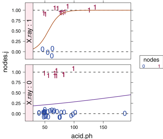
Fig. 17.17 Figure 17.13 plus fitted logistic curves for the interaction model glm(nodes \sim X.ray * acid.ph, data=lymph, family=binomial) .
