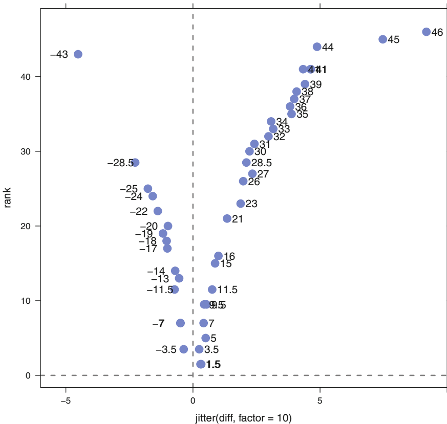
Displayed numbers are the signed-ranks. Tied ranks are shown by average rank and overstrikes.
