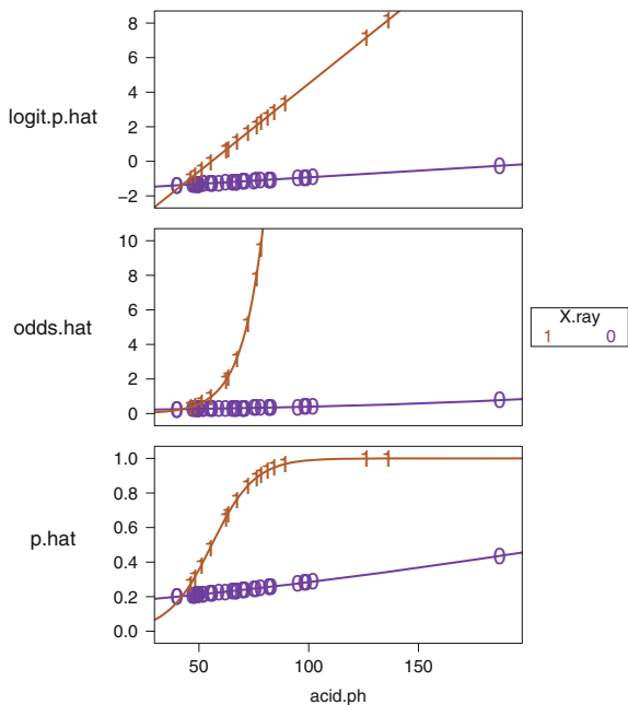
Fig. 17.18 Three scalings of fit to nodes \sim X.ray * acid.ph with the responses at both values of X.ray superposed on the same plot. The non-parallel lines in the logit.p.hat panel show the analogy with interaction in the ANCOVA setting. Two of the points in the odds.hat panel are beyond the limits we chose for the display. Their values in the odds.hat scale are 1256 and 3472.
