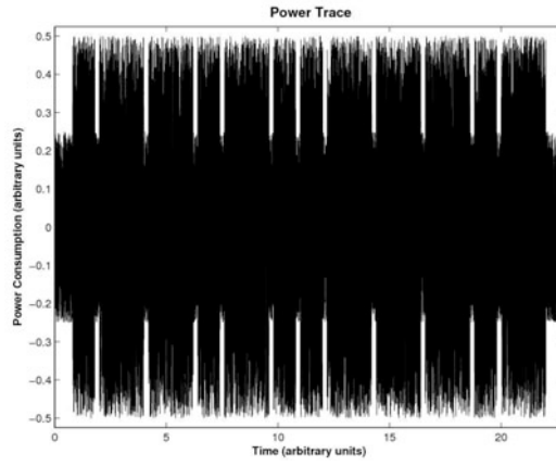
Fig. 7.5 Power consumption of an RSA decryption
