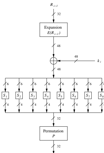
Fig. 3.8 Block diagram of the f -function
